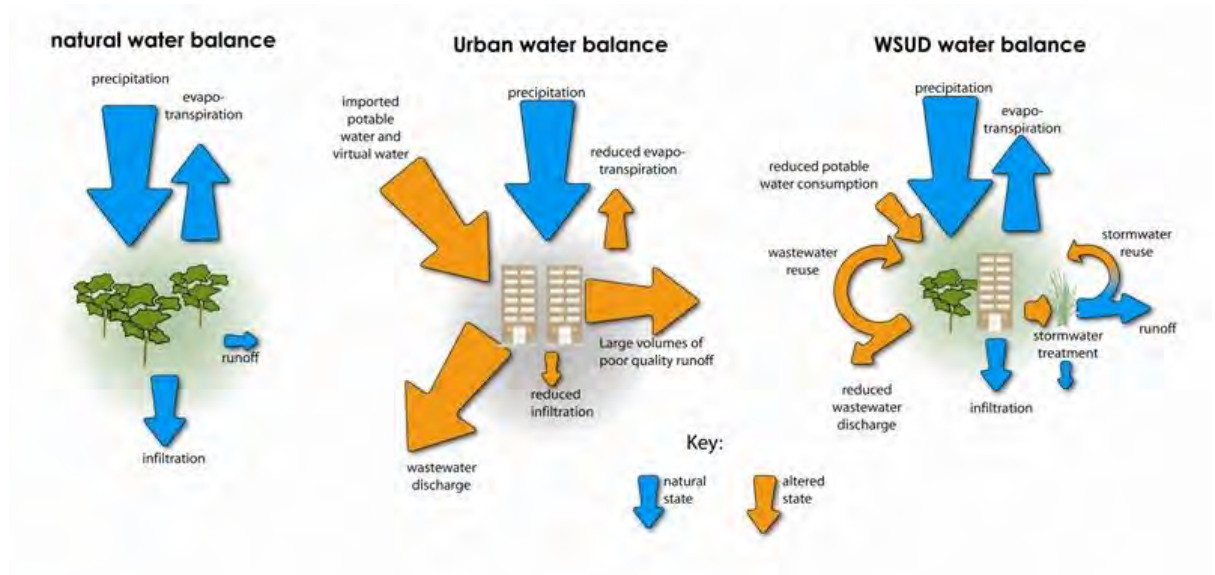
Figure 9: How the water cycle works in natural and urban areas ( SEQ Healthy Waterways Partnership, 2010 )
