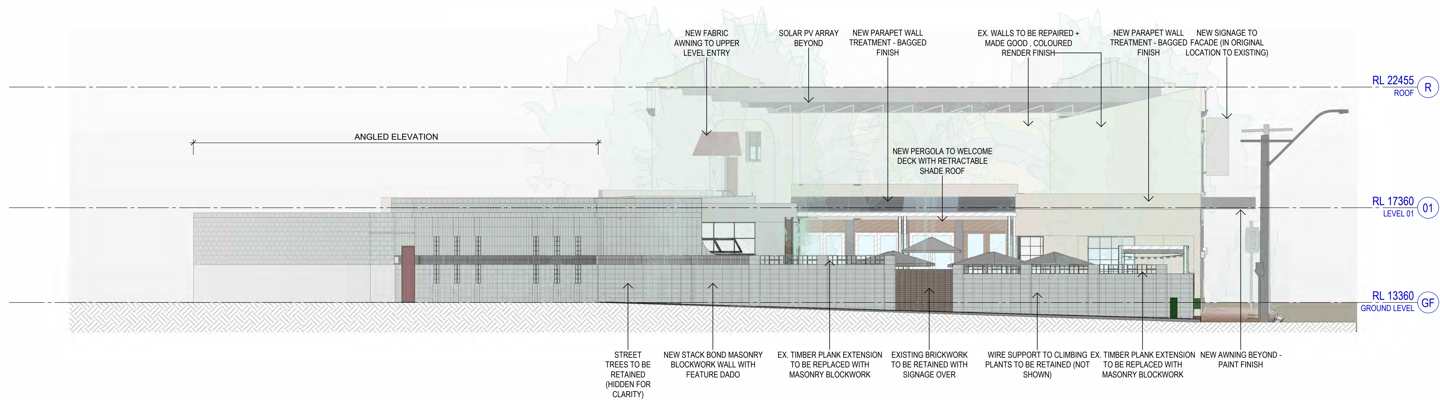
NORTH-EAST ELEVATION Northern Carpark
