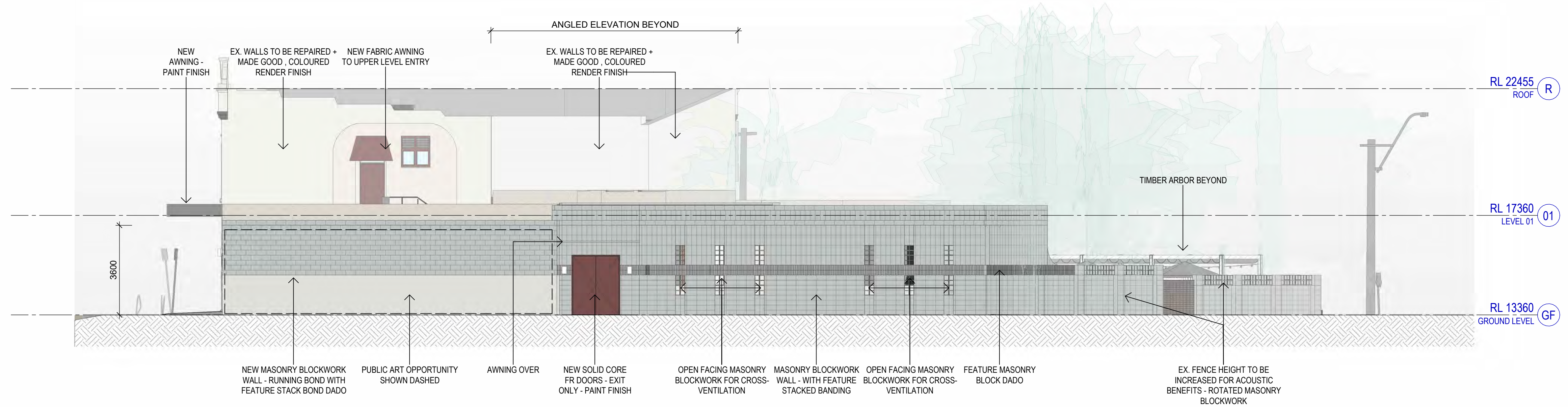
EAST ELEVATION Eastern Carpark
